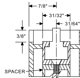
SECTION YY
